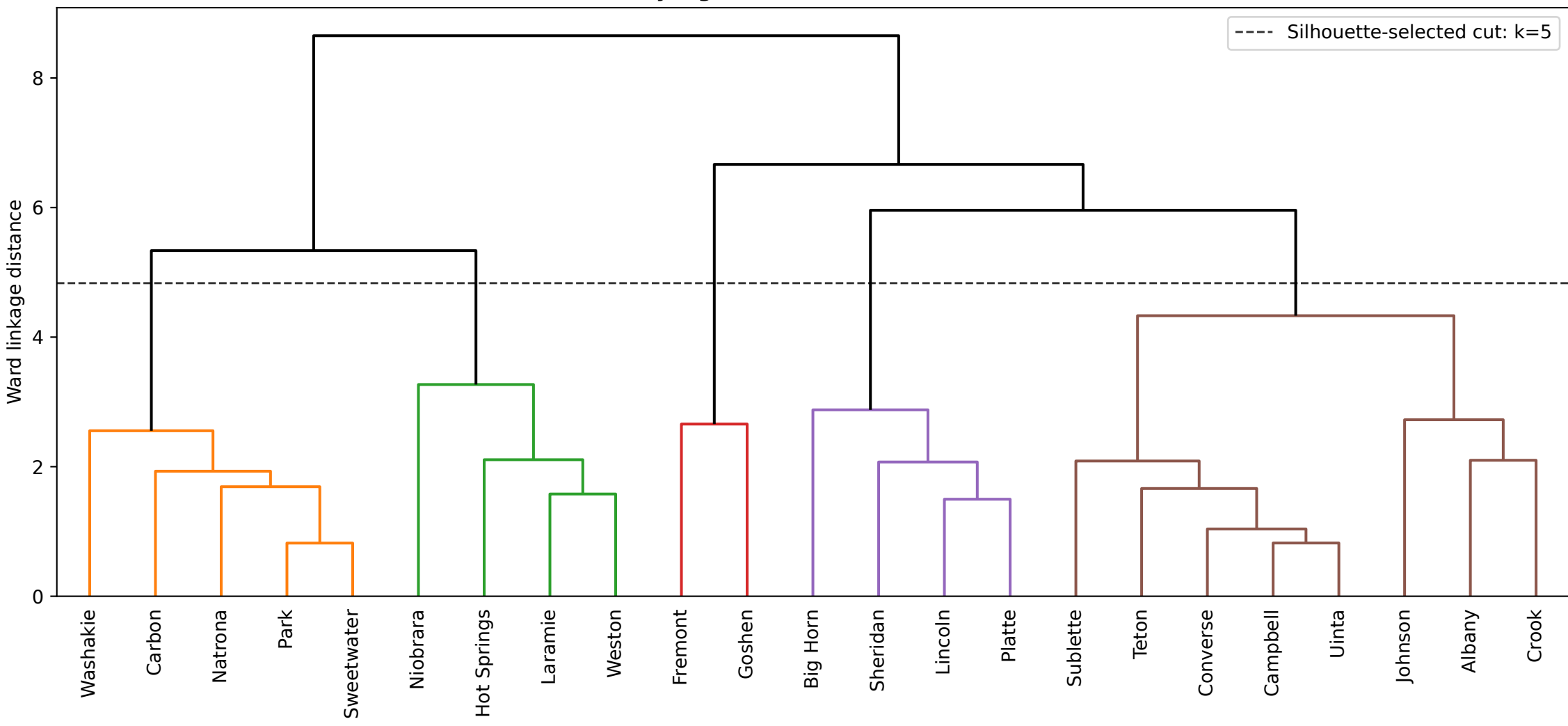
Ward Dendrogram — Simplified 6-Feature Space, 28-day Sakoe-Chiba Band Branch colors forced by highest silhouette score: k=5, silhouette=0.272
